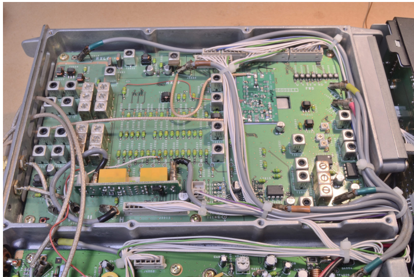
Fig 1 – General view of PAT inside FT847
