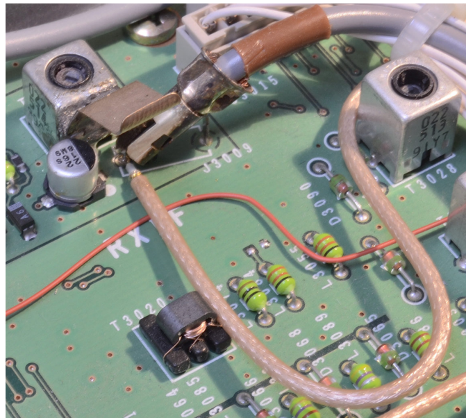
Fig 3 – Coax connection at J3009 for PAT
