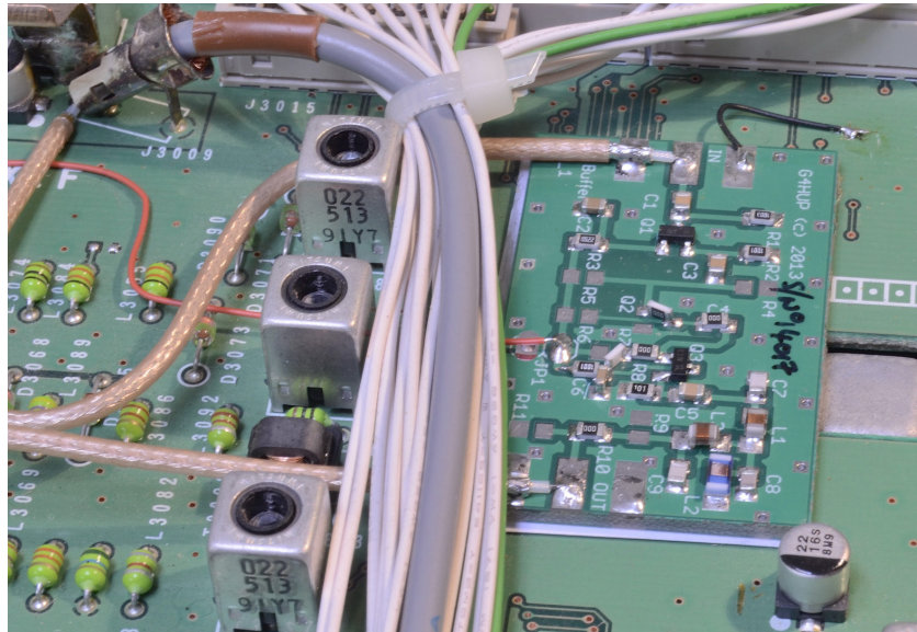
Fig 4 – Close up of PAT board installed, showing coax terminations and 0V connection to RF PCB
