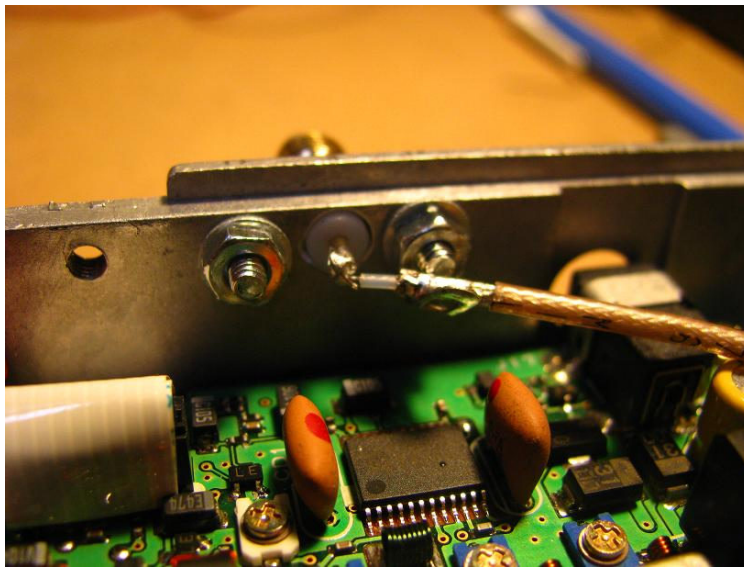
Fig 7 – Correct method of termination for the RG178 cable
