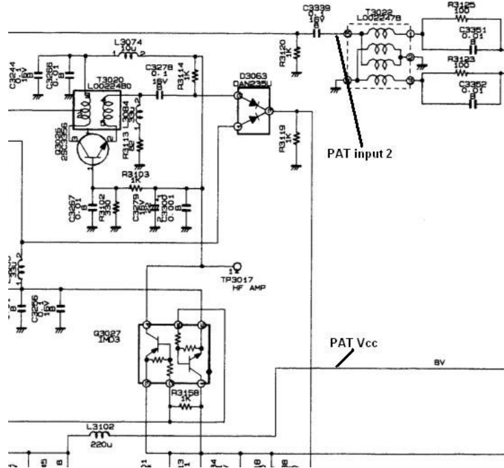
Fig 5 – PAT input for 2 nd Rx function – other connections also shown
