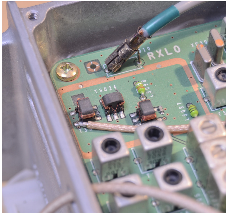
Fig 6 – Connection to T3022 for 2 nd Rx function
